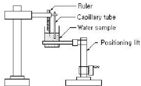
Fig. 13. Schematic diagram of the surface tension measurements.
