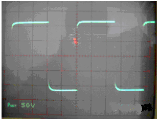
Fig. 5. 12 volts of square wave signal captured by an oscilloscope for electrode devices.
