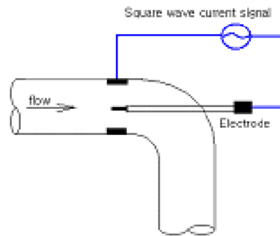
Fig. 3. Schematic diagram of the metal electrode device.
