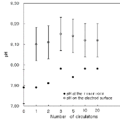
Fig. 12. Variations of pH according to the number of cooling water circulations.
