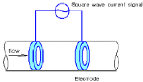
Fig. 4. Schematic diagram of the graphite electrode device.
